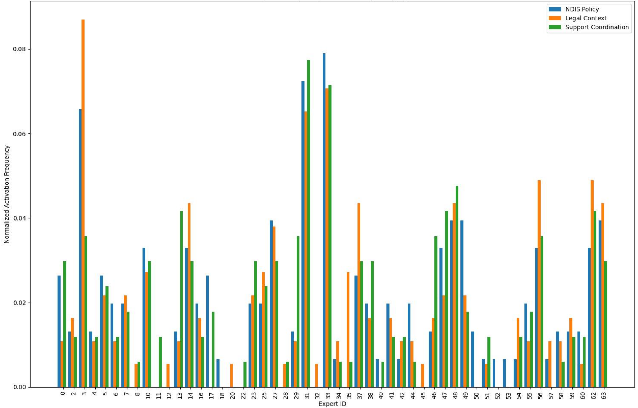
Layer 4 - Expert Specialization by Category
