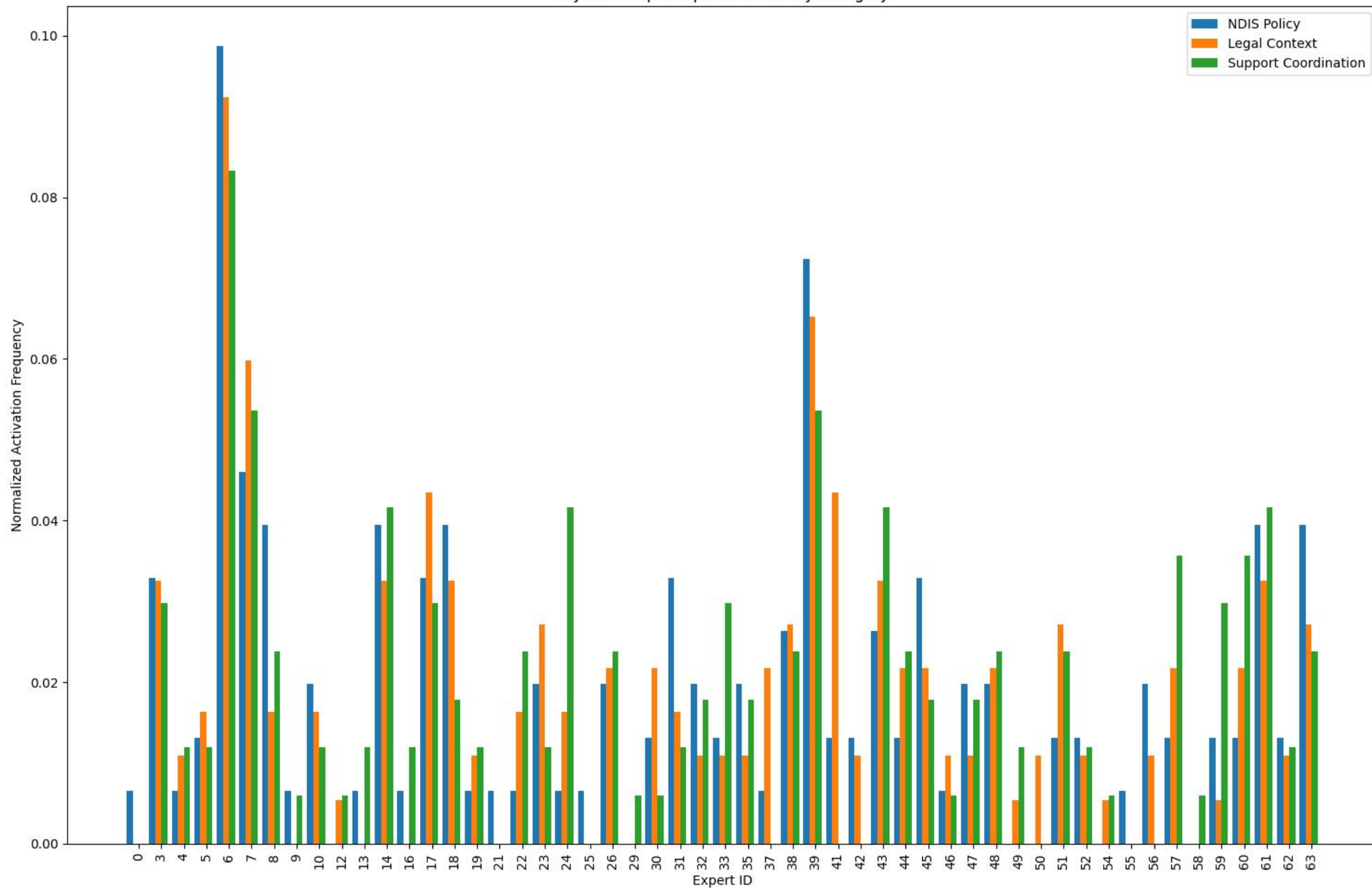
Layer 0 - Expert Specialization by Category
